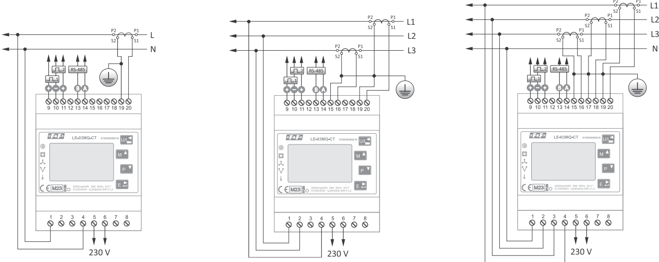
230 V AC 1-phase 2-wire installation 3×400 V 3-phase 3-wire inst. (without neutral wire) 3×230 V+N 3-phase 4-wire installation
