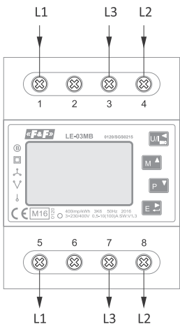
3×400 V 3-phase 3-wire installation (without neutral wire)
