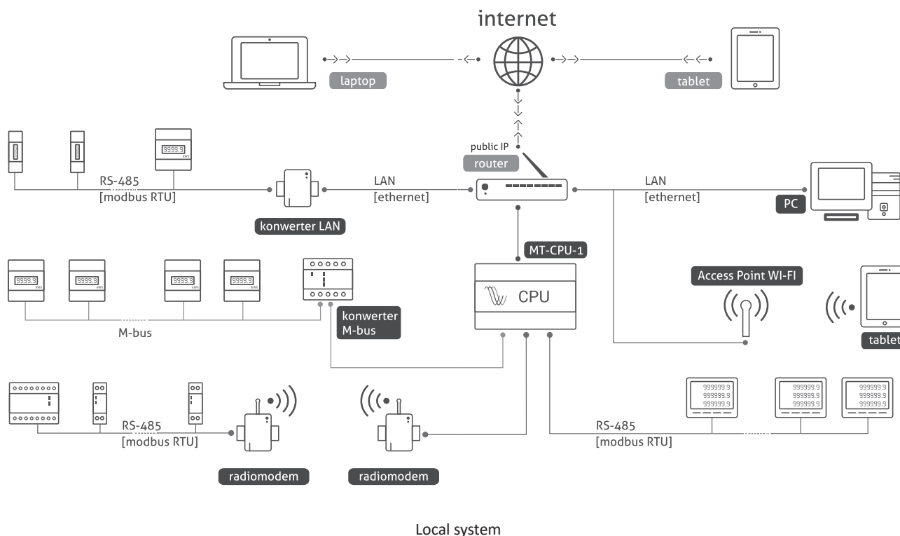
Local system
