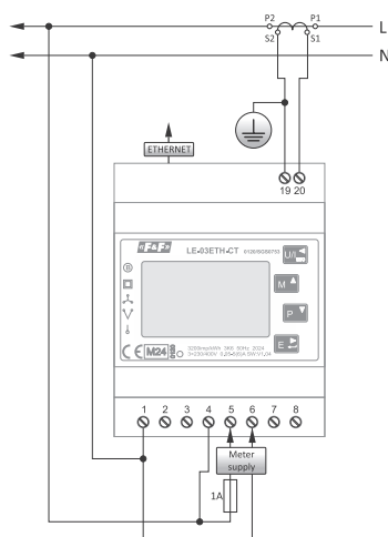
230 V AC 1-phase 2-wire installation
