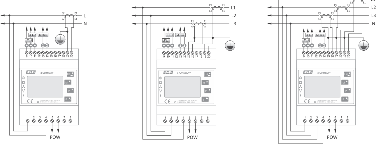
230 V AC 1-phase 2-wire installation 3×400 V 3-phase 3-wire inst. (without neutral wire) 3×230 V+N 3-phase 4-wire installation
