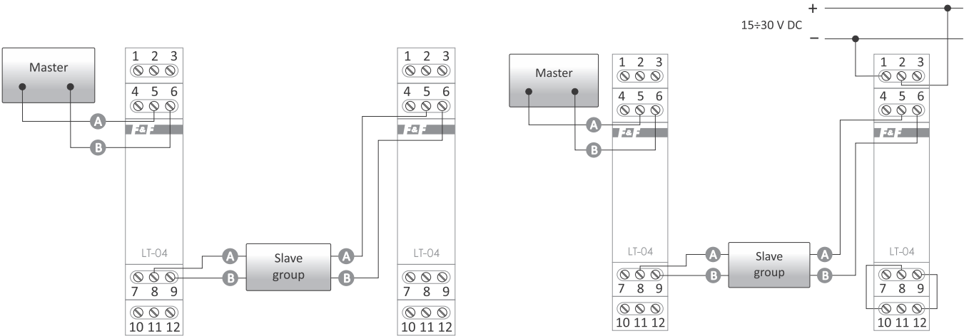
Network termination system
