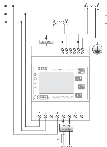
3×400 V 3-phase 3-wire inst. (without neutral wire)
