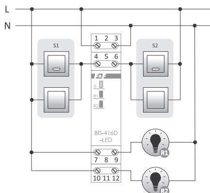
Example of connection with control pulse N
