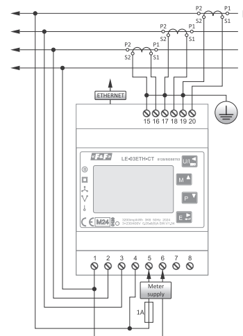
3×230 V+N 3-phase 4-wire installation
