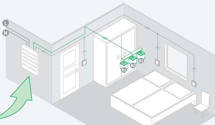
Example of a lighting system for controlling the light intensity by switching on sections R1 and R2 respectively
